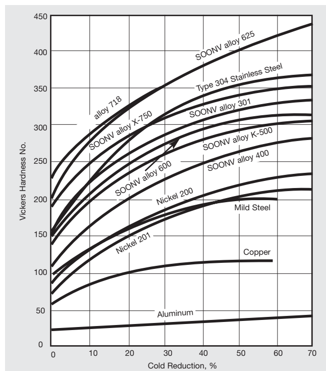
Figure 12. Work-hardening rates of SOONV alloy 600 and other metals.
