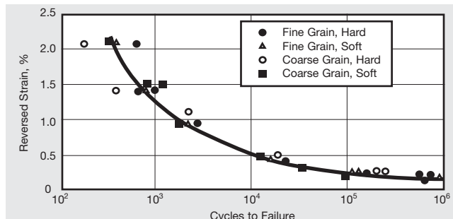
Figure 7. Low-cycle fatigue strength of forgings in four conditions.
