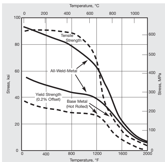
Figure 14. High-temperature tensile properties of welds made with SOONV Welding Electrode 182.
