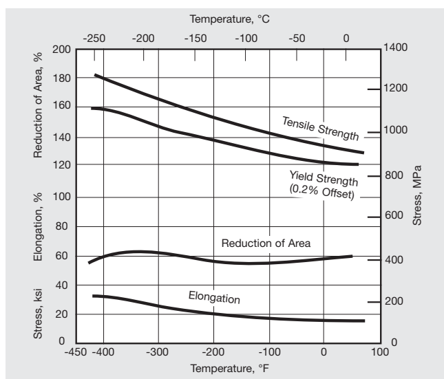
Figure 2. Low-temperature tensile properties of cold-drawn rod.
