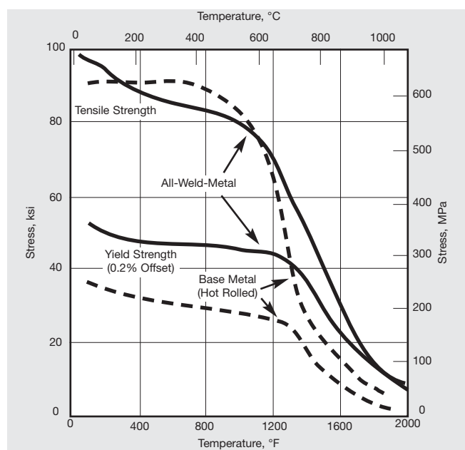
Figure 13. High-temperature tensile properties of welds made with SOONV Filler Metal 82.
